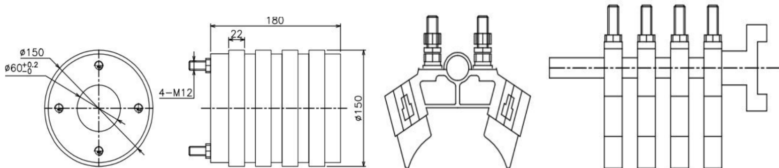
Collector ring
